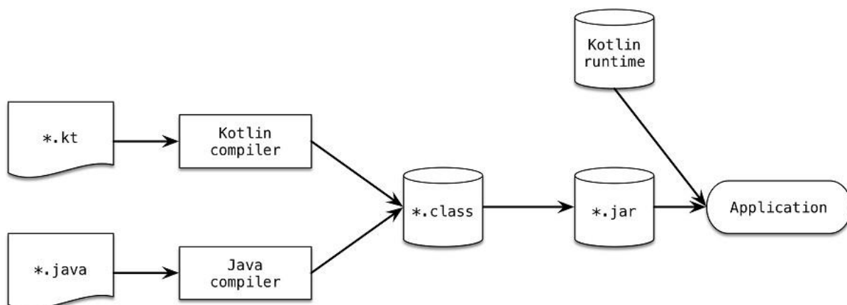
Figure 1.1 Kotlin Build Process
