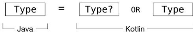
Figure 6.9 Java types are represented in Kotlin as platform types, which you can use either as a nullable type or as a non-null type.
